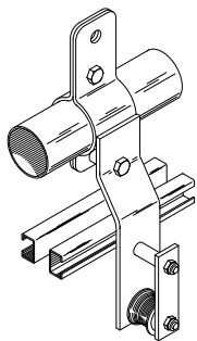
No. 1021 BLACK IDLER PULLEY
