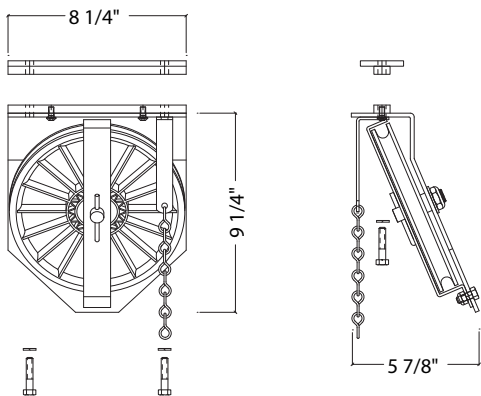
1024 SINGLE END PULLY
