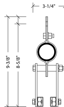
No. 1010 BLACK TRACK
