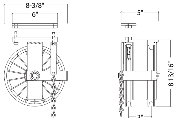
1023 DOUBLE END PULLY
